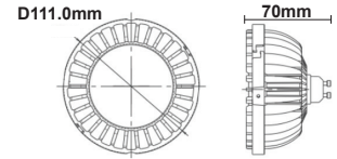
Dimension ( mm )
